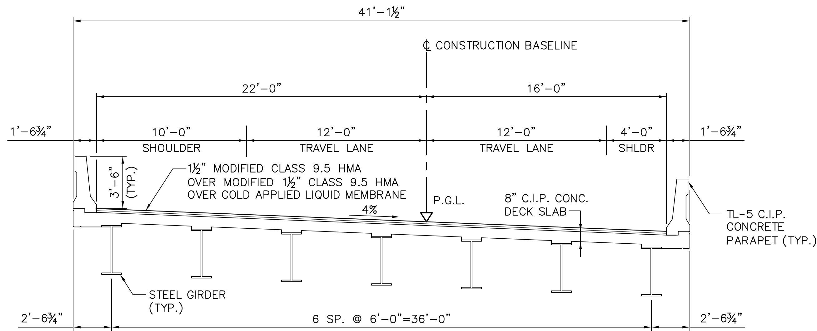
TRANSVERSE CROSS SECTION
