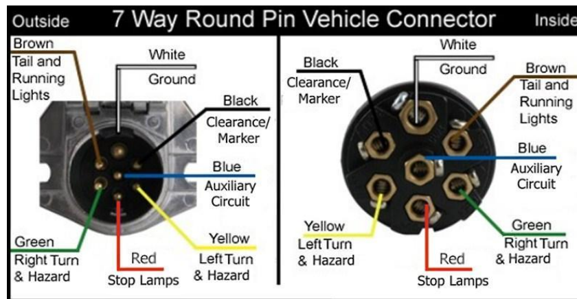
RIDOT Standard Truck Wiring Diagram
